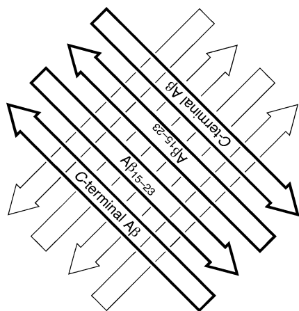
Figure 6. Cartoon of an eight-stranded cruciform oligomer comprising the A\beta_{15-23} and C-terminal \beta -strands.
